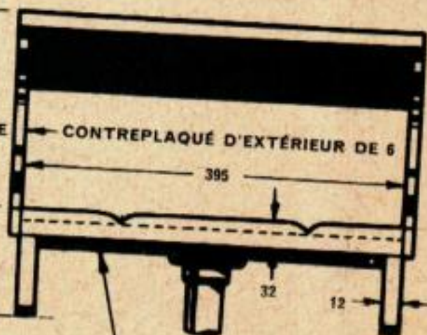
TRAVERSE 12 x 150 x 365
