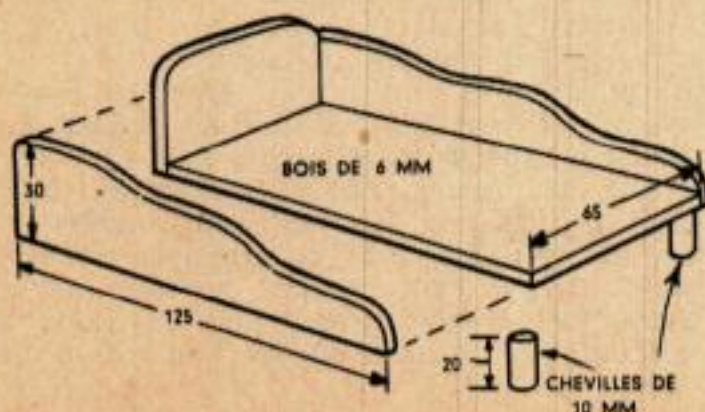
SERVANTE A CIGARETTES
